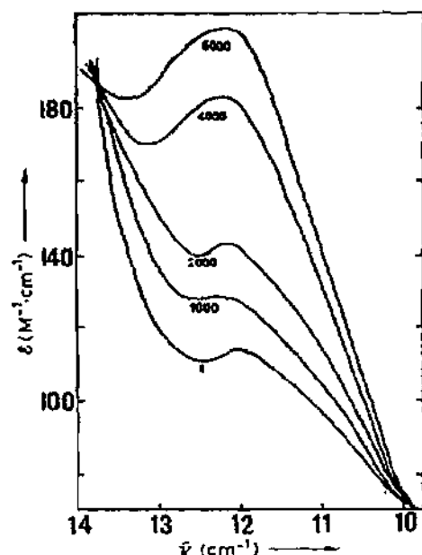
Fig. 8. Pressure dependence of the spectrum of nickel (II) N,N' -di-2-naphthylaminotroponoiminate in \text{CH}_2\text{Cl}_2 in the range 1–6000 atm.
