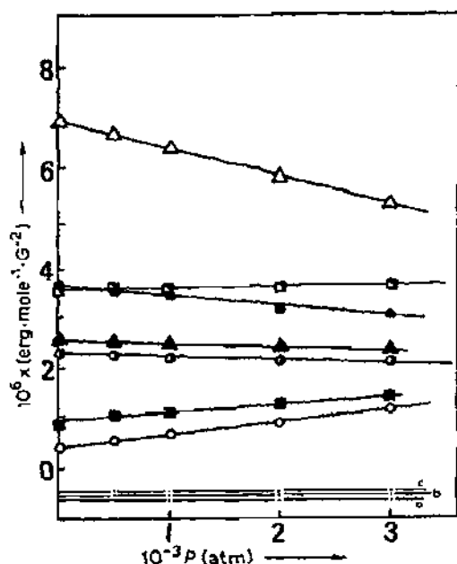
Fig. 7. Pressure dependence of magnetic susceptibility. ( \Delta ) Tris ( N,N -di- n -butylthiocarbamato) iron (III) in \text{CHCl}_3 ; ( \bullet ) bis( N -phenylsalicylaldimino) nickel (II) in \text{CHCl}_3 ; ( \circ ) bis( N,N' -diethylamino-troponeimineato) nickel (II) in \text{CHCl}_3 ; ( \blacktriangle ) tris( N -ethylxanthato) iron (III) in \text{CHCl}_3 ; ( \ominus ) tris( N -methyl-xanthato) iron (III) in \text{CHCl}_3 ; ( \bullet ) bis( N,n -heptylsalicylaldimino) nickel (II) in \text{CH}_2\text{Cl}_2 ; ( \circ ) bis( N,n -propylsalicylaldimino) nickel (II) in \text{CHCl}_3 ; a, b, c – common solvents, \text{CHCl}_3 , \text{CH}_2\text{Cl}_2 and (\text{CH}_3\text{OH})_2 respectively.
