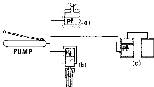
Fig. 4. Piston and cylinder pressure devices (schematic). Compressed fluid is pumped into cylinder to apply pressure to surface indicated by "P". (a) Pressure intensifier using large primary and small secondary piston areas. (b) Application of pressure with intensification, to fluid in a secondary cylinder with a locking nut for retaining the pressure after removal of the primary (larger) piston. (c) Phase separation of two potentially interacting fluids.
