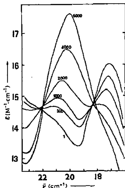
Fig. 10. Pressure dependence of \text{NiL}_2(\text{NO}_2)_2 in the range 1–6000 atm where \text{L} = N,N' -diethylenediamine. The band near 20,000\text{ cm}^{-1} is due to the nitro form of the complex.
